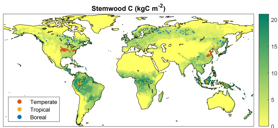
Figure 1. Location of the grid cells included in calibration simulations (100 per FPFT). The map shows simulated stemwood C ( \text{kgC m}^{-2} ) for a simulation with potential natural vegetation.
